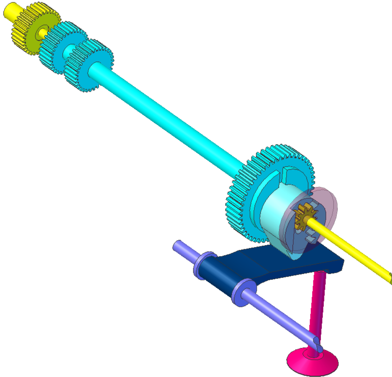
I.C.E. Valve Cam Timing & Throw Driving Mechanism
